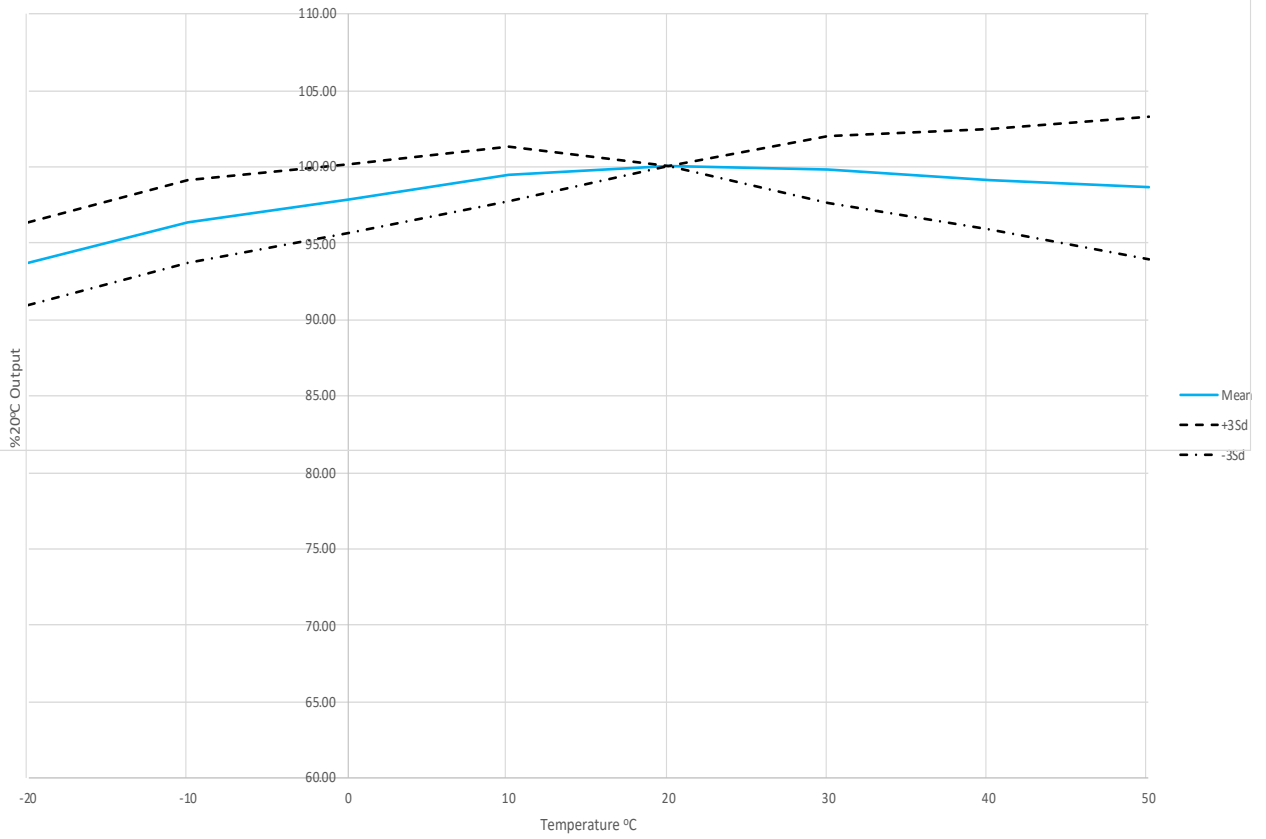
GS+4CL2 %20°C Output vs Temperature °C
